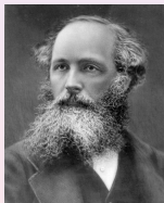
Maxwell
